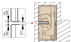
Min. 2 mm gap between door & jamb 門和門框之間最少要有 2 mm 間隙
